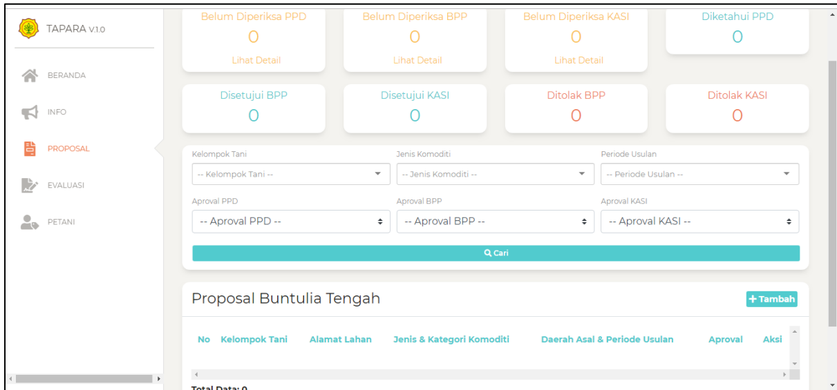
Gambar 7.1. Halaman Proposal
