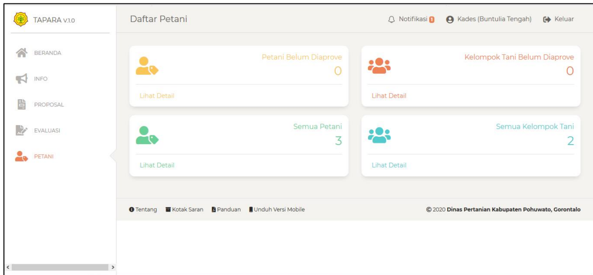
Gambar 6.1. Halaman Petani
