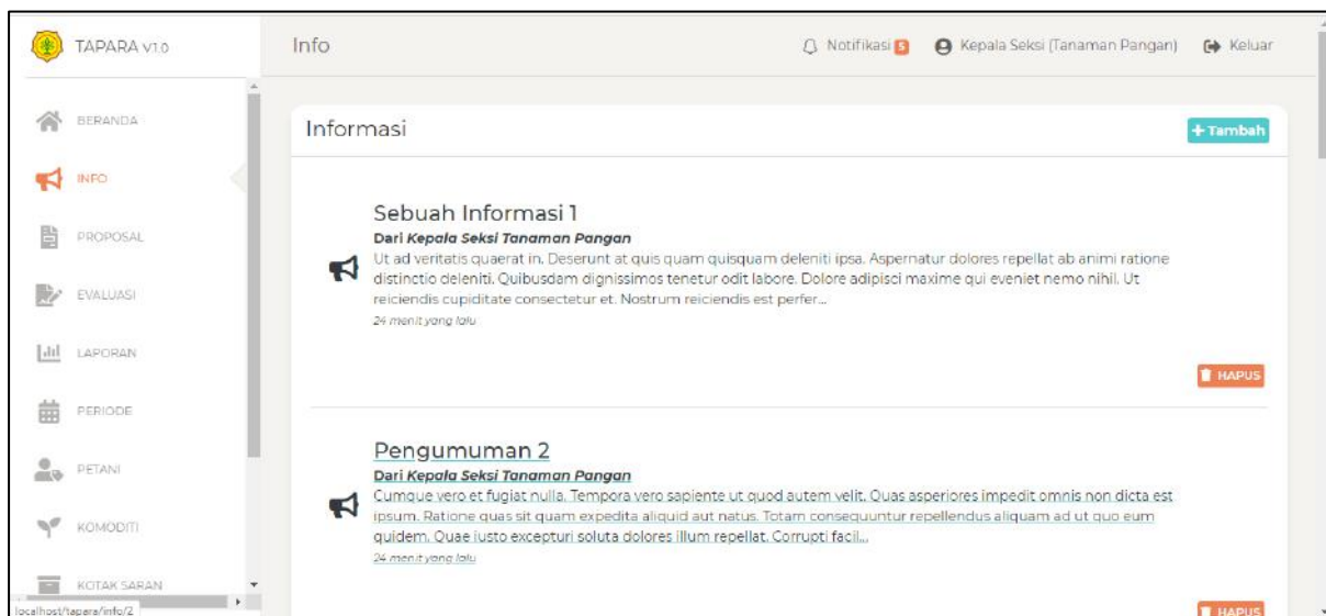
Gambar 5.1. Halaman info
